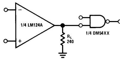
Driving TTL
